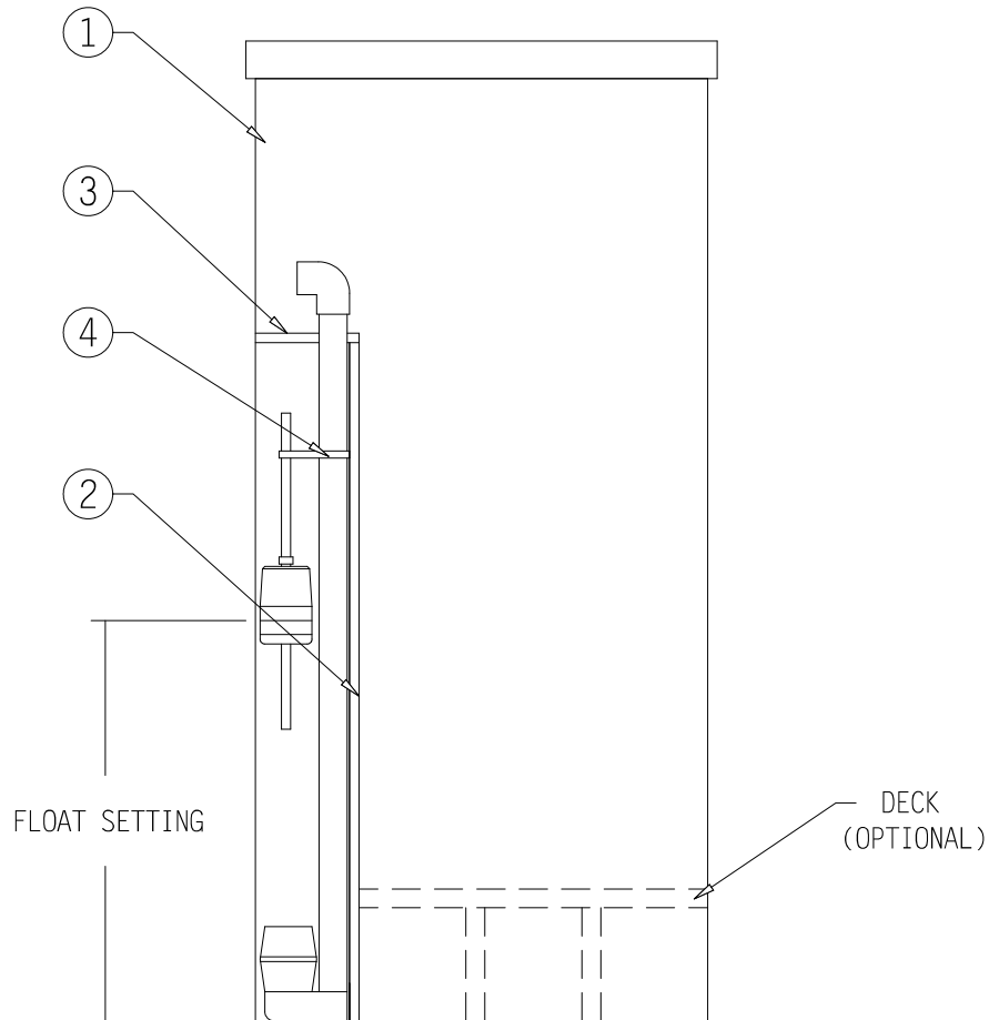
24" x 50" BRINE TANK POLYETHYLENE
